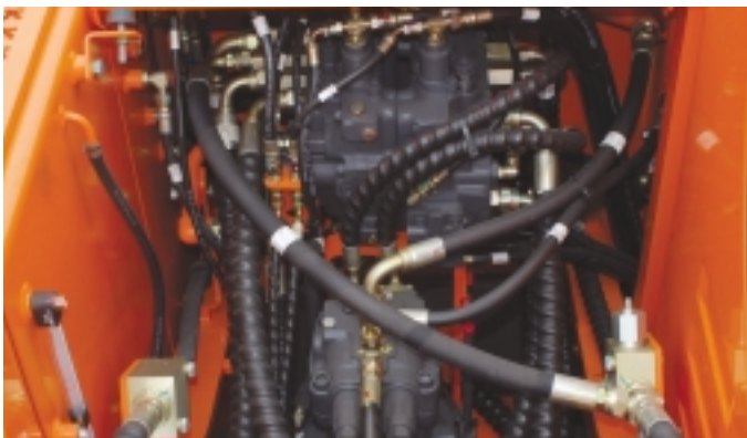
Swing drive
